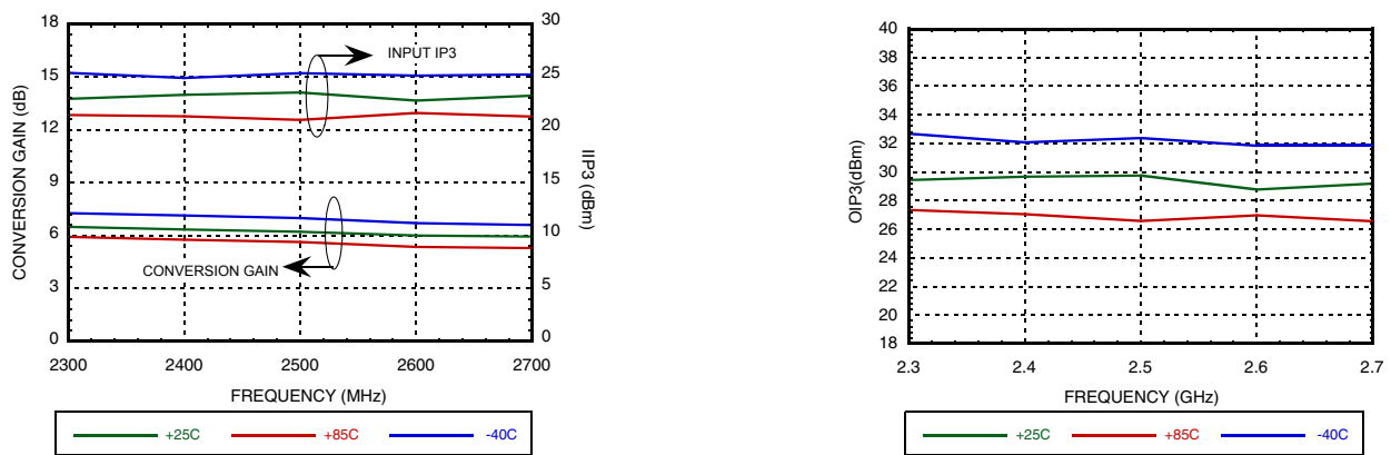
Figure 79. Conversion Gain, IIP3 and OIP3 for 2500MHz RF frequency bands. [1]
