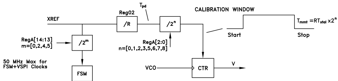
Figure 68. VCO Calibration
