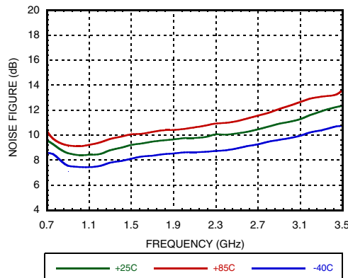
Figure 26. Noise Figure vs. Temperature @ VGATE=4.9V
