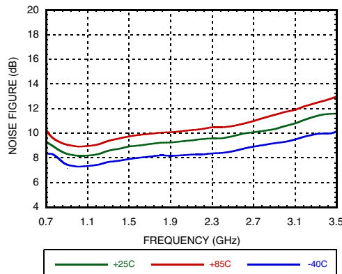
Figure 31. Noise Figure vs. Temperature @ VGATE=4.8V
