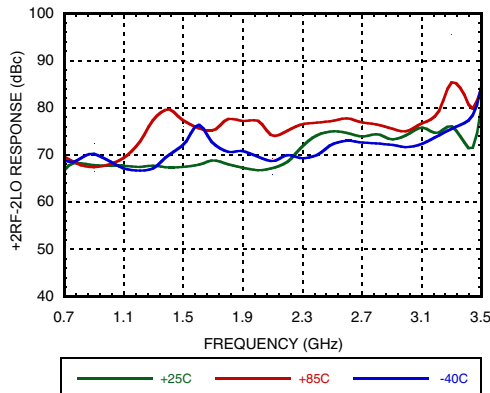
Figure 29. +2RF -2LO Response vs. Temperature @ VGATE=4.8V
