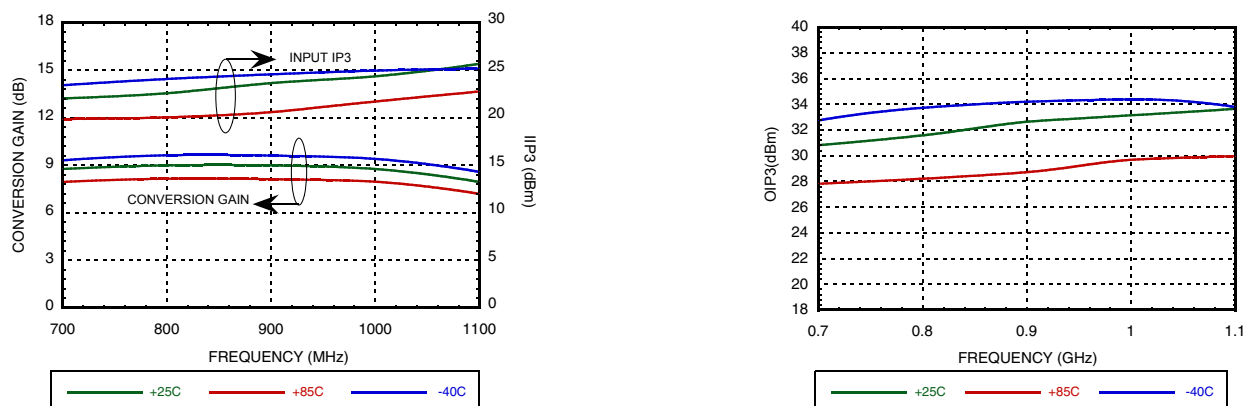
Figure 77. Conversion gain, IIP3 and OIP3 for 900MHz RF frequency band. [1]
