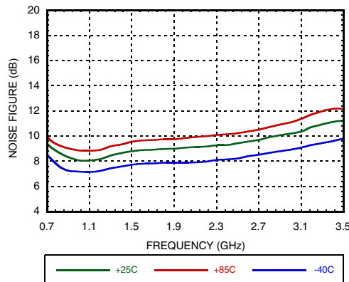
Figure 36. Noise Figure vs. Temperature @ VGATE=4.7V
