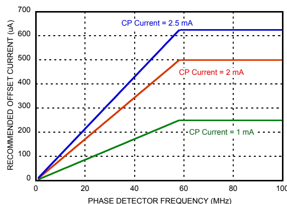
Recommended CP offset current vs PD frequency for typical CP gain currents. Calculated using (EQ 9)
