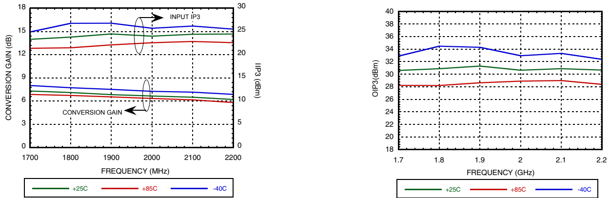
Figure 78. Conversion Gain, IIP3 and OIP3 for 1900MHz RF frequency band. [1]
